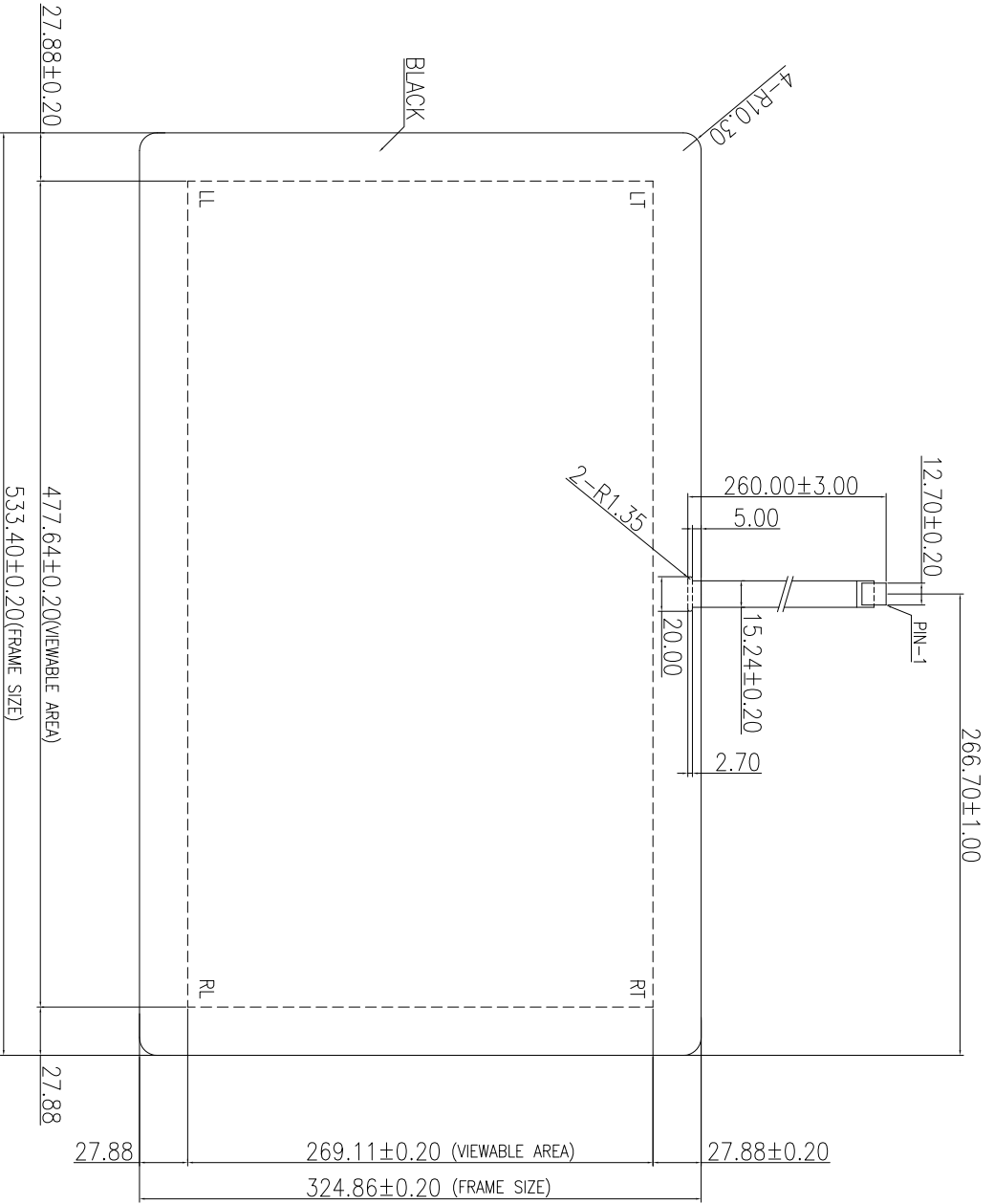
FRONT VIEW
